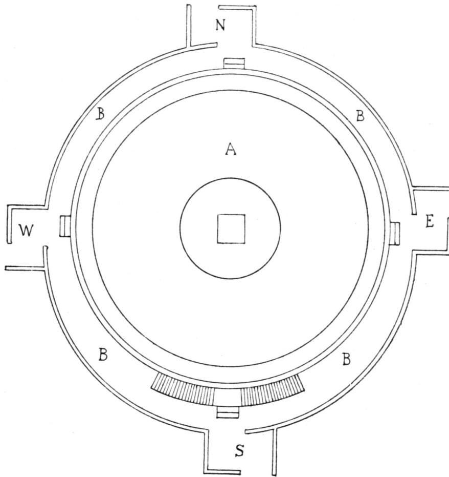
14: Fig. 13. — Plan of the Sâncchi Stûpa. A , Dome, or body of Stûpa. B B B B , Procession Path round the Stûpa. N E S W , Gateways or entrances to Procession Path at each of the cardinal points.
