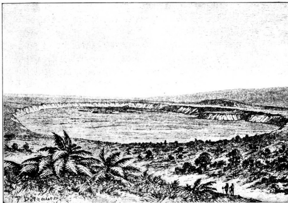
9: Fig. 9. — Kilaueas krater, Hawai.
