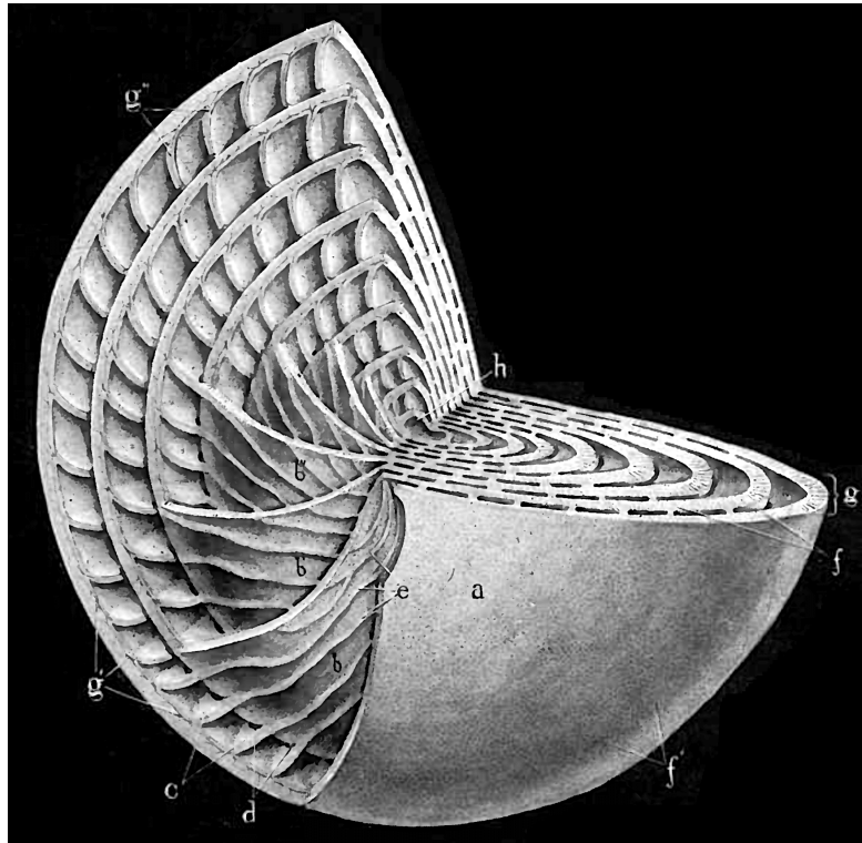
FIGURE 16 — DIAGRAM OF A NUMMULITE TO SHOW PERPENDICULAR AND TRANSVERSE SECTIONS IN ONE VIEW.
