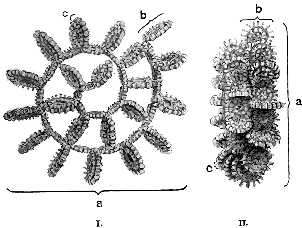
FIGURE 10A — DIAGRAMMATIC FIGURES ILLUSTRATING THE SPIRODISCOID CHARACTER OF THE MINUTE STRUCTURE OF THE NUMMULITE SKELETON OR SHELL.
