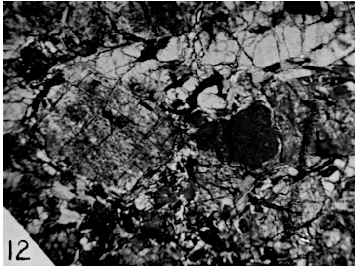
24: Plate 2D: Figure I2 — Cornish granite. Rhomboidal feldspar crystal to left of center shows \frac{1}{8} inch (3 mm.) above middle of lower left border and well between two parallel dark streaks a spiral rim (1 mm. diam.) with cog-like light and dark flecks. On left are two much larger concentric rims with radial “septa” and “alars.” The upper dark streak, nearly tangential to inner of these, stabs five septa, 3x. Lens necessary.
